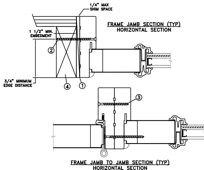
THROUGH FRAME INSTALLATION
